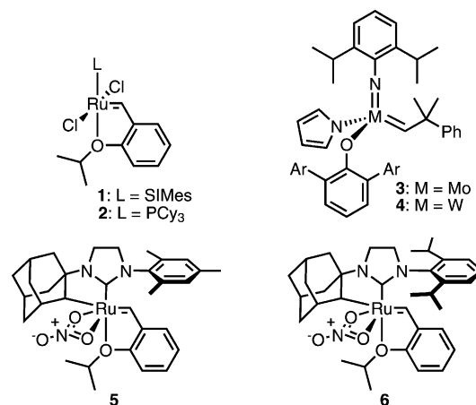
Scheme 1. Prominent olefin metathesis catalysts (Ar = 2,6-(2,4,6- i Pr 3 C 6 H 2 ) 2 C 6 H 3 ; SiMes = 1,3-Bis(2,4,6-trimethylphenyl)-4,5-dihydroimidazol-2-ylidene).
