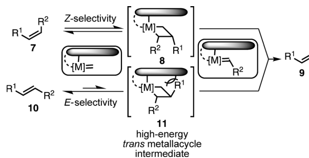
Scheme 2. Destabilized trans -metallacyclobutane 11 , which disfavors metathesis of E -olefins.
